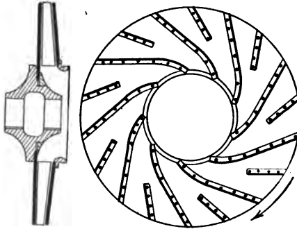
FIG. 96.—Jaeger's patent impeller.
